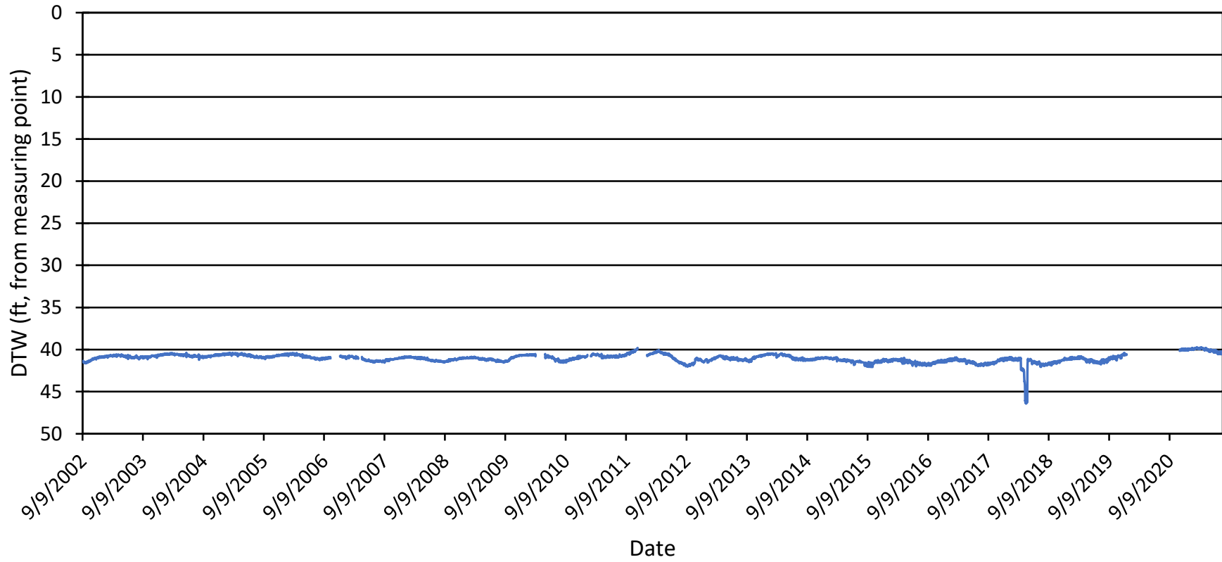
AVG_KCSD (9/9/2002 to 7/27/2021)
