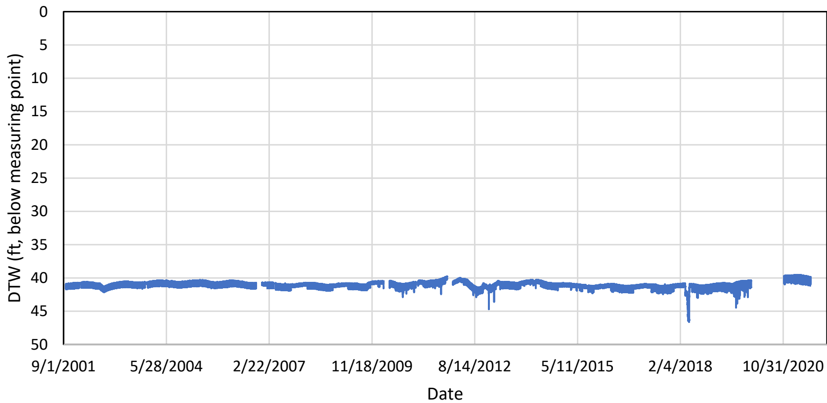
KCSD_WELL (9/25/2001 to 7/27/2021)
